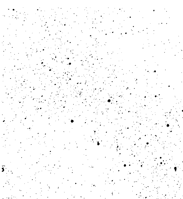
FIG. 4. MILKY WAY.
