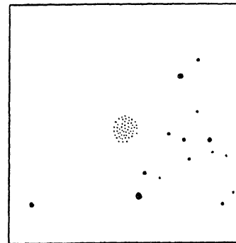
17^{\text{h}} 17^{\text{m}}.1 \quad -26^{\circ} 15'
