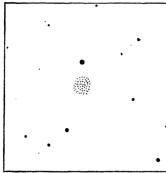
0^{\text{h}} 29^{\text{m}}.2 \quad -9^{\circ} 00'
