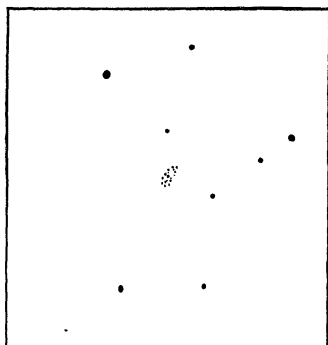
1^{\text{h}} 54^{\text{m}}.2 \quad -6^{\circ} 30'
