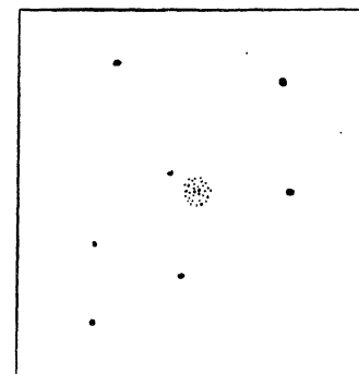
1^{\text{h}} 47^{\text{m}}.7 \quad -14^{\circ} 17'
