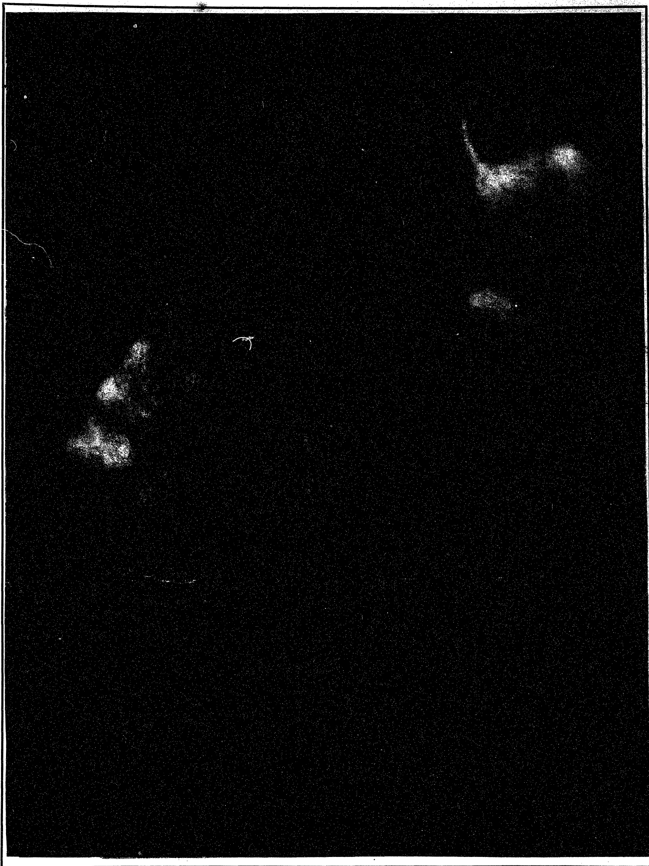
CENTRAL PART OF THE NEBULA IN ORION.
